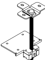
Zipnut (Drywall) Ceiling Mount (575/675 – Flush)
